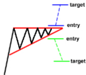
Ascending Triangle
