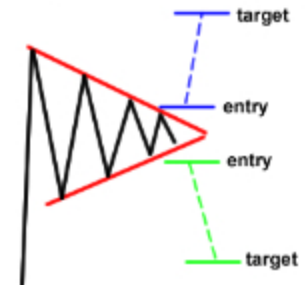
Symmetrical Triangle
